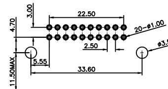
APPLICABLE P.C.B LAYOUT(REF.) P.C.B THICKNESS t=1.6mm
