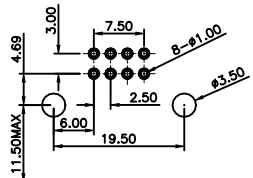
APPLICABLE P.C.B LAYOUT(REF.) P.C.B THICKNESS t=1.6mm
