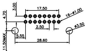
APPLICABLE P.C.B LAYOUT(REF.) P.C.B THICKNESS t=1.6mm
