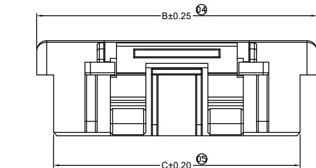
2*06P~2*14P Shape Scale 1:1
